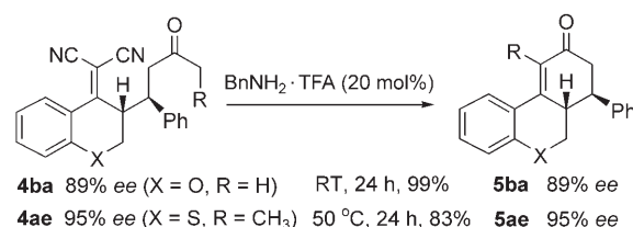
Scheme 5. Domino Michael–retro–Michael reactions promoted by an achiral primary aminocatalyst.
